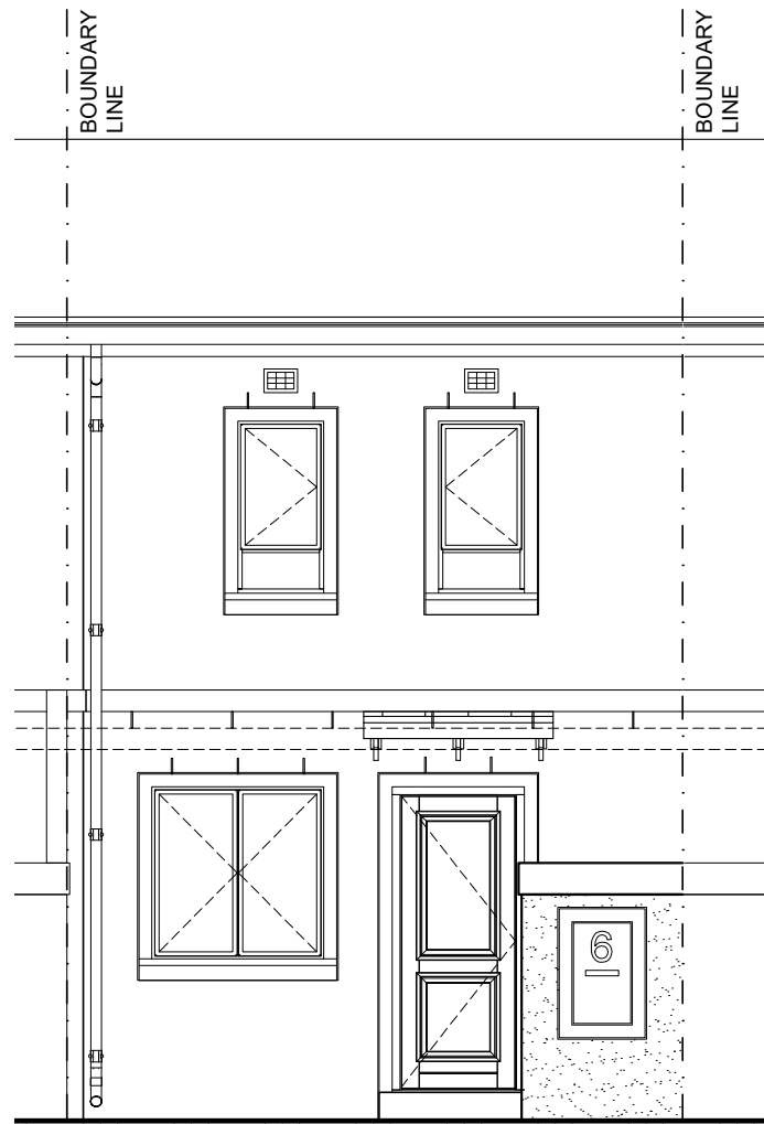
TYPICAL STREET ELEVATION
