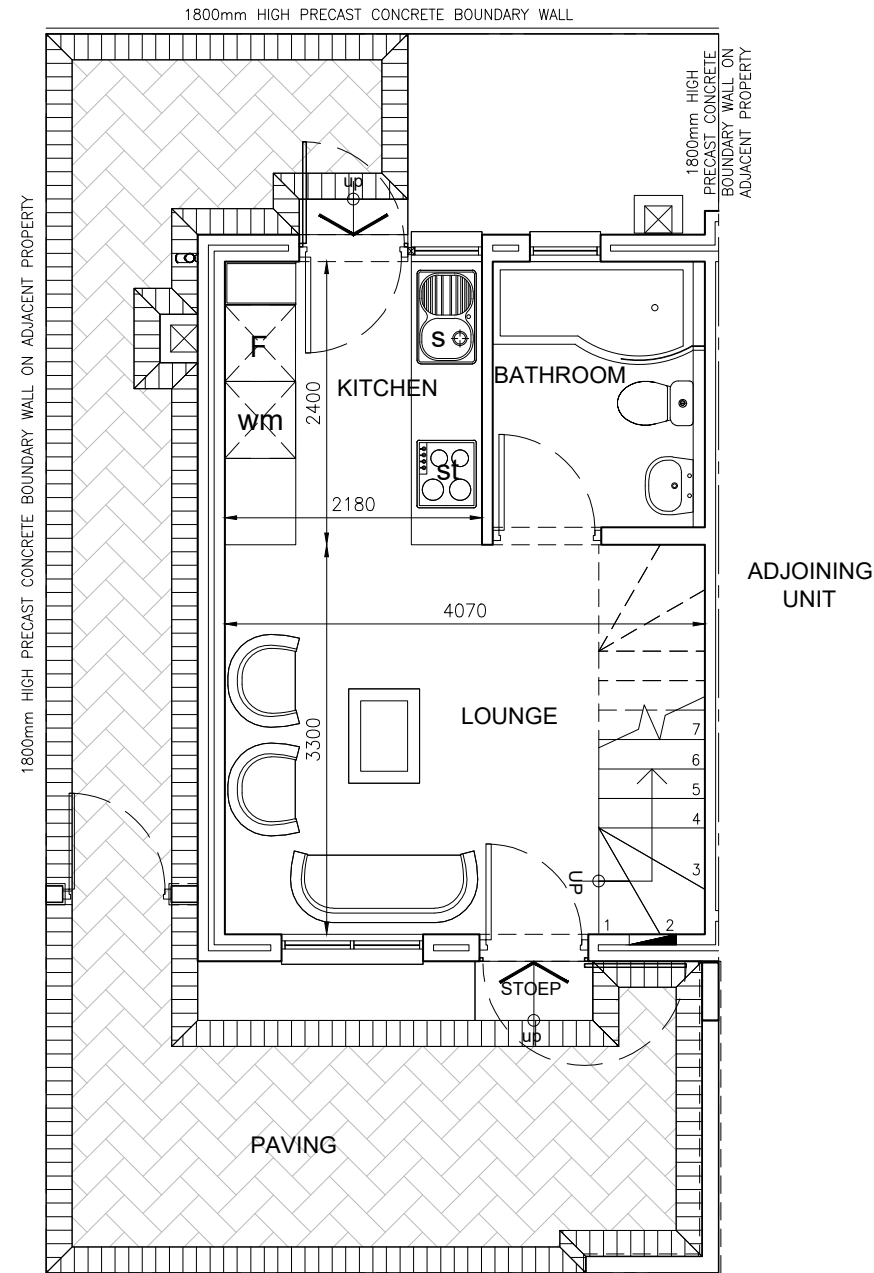
GROUND STOREY PLAN
