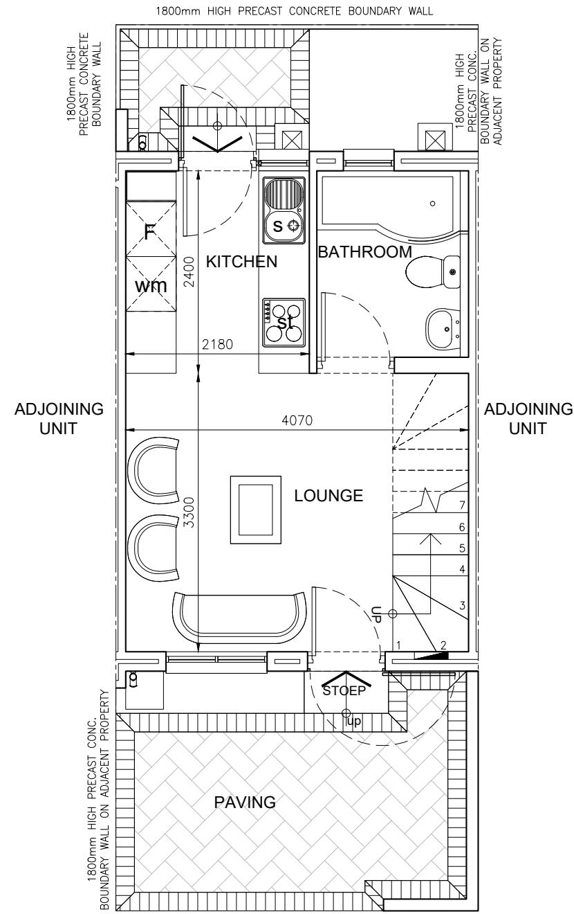
GROUND STOREY PLAN
