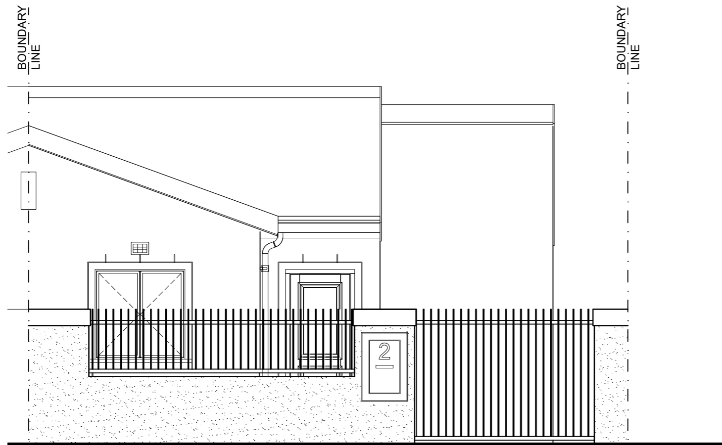
TYPICAL STREET ELEVATION
